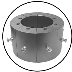
Adapter Die Set 160mm OD to 99mm ID (Included) P/N:104618
