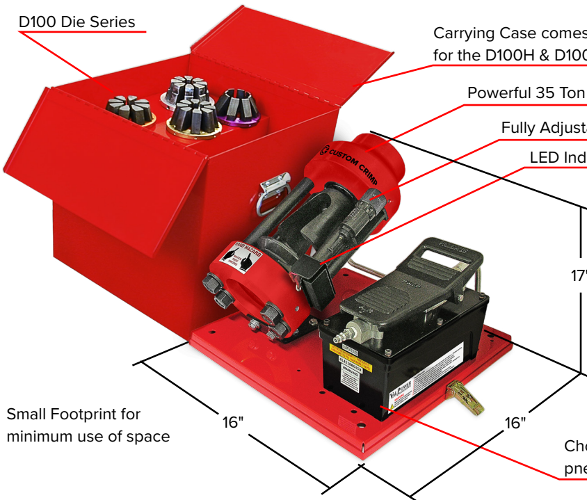
Pneumatic Pump (Optional) P/N:VAP-10-100
