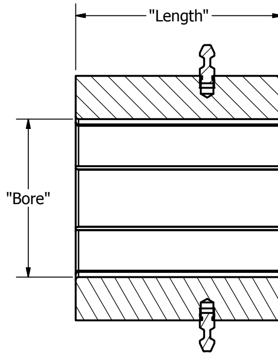
SECTION H-H SCALE 1 / 2
